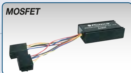
5/207 15 Ampère Peak ISO CONNECTOR Packed 1 pc.
