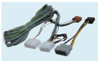
4/742 CHRYSLER Voyager '05>'07 Con amplificatore / With amplifier Power and speakers Packed 1 pc.
