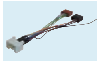
4/743 PEUGEOT 4007 '07> Senza navigatore e amplificatore Without navy and amplifier Power and speakers Packed 1 pc.
