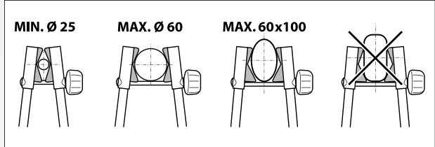
ART. 319C - 319CP CHIUSURA CON POMELLO CLOSE-UP WITH KNOB
