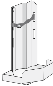
Cod. 91251 Portaestintore lamiera zincata regolabile da ø 160 a 220 mm. ± 2 mm. Zinc plated adjustable extinguisher-holder from ø 160 to 220 mm. ± 2 mm.
